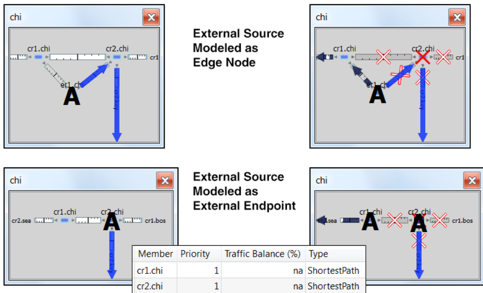
Figure 15-3 Example External Demand Source
