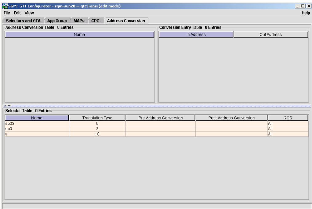
Figure 3-73 GTT Configurator, Showing Address Conversion Tab
