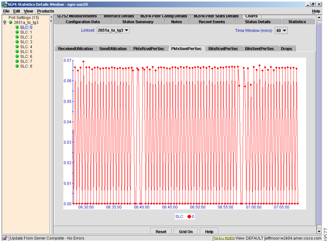
Figure 3-43 PktsSentPerSec Chart for a Link
