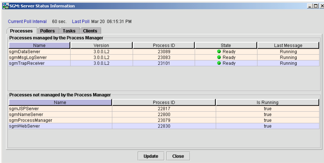
Figure 3-62 Server Status Information Window
