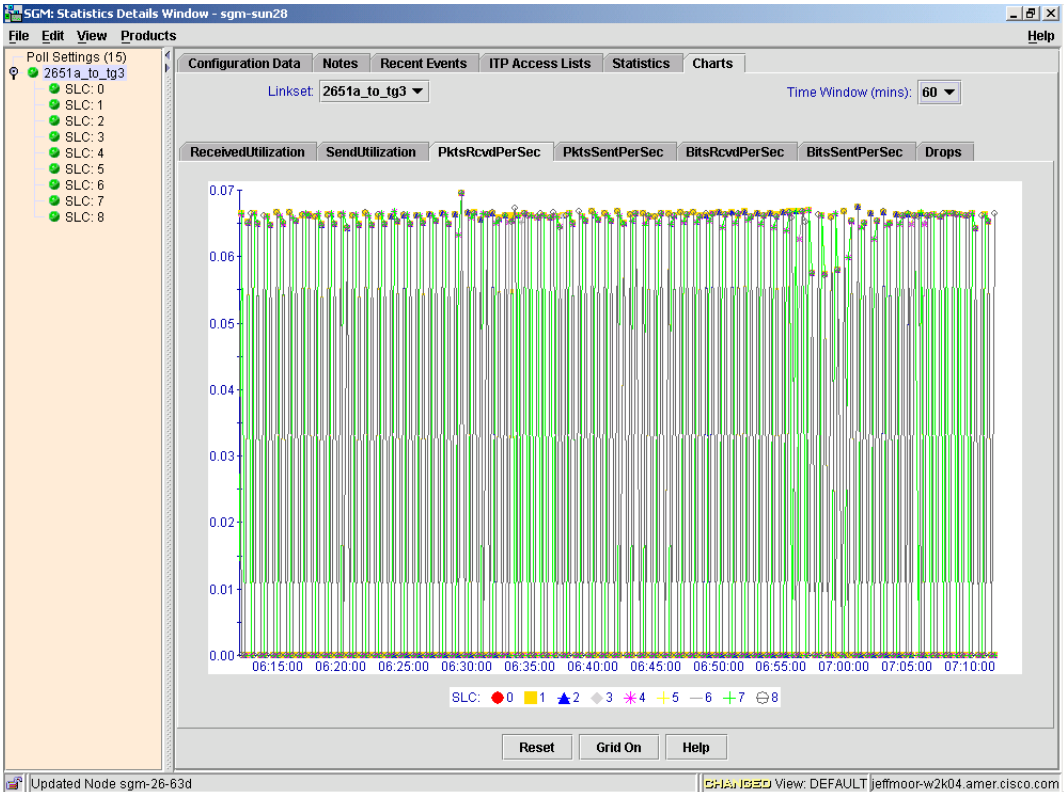
Figure 3-16 PktsRcvdPerSec Chart for a Linkset
