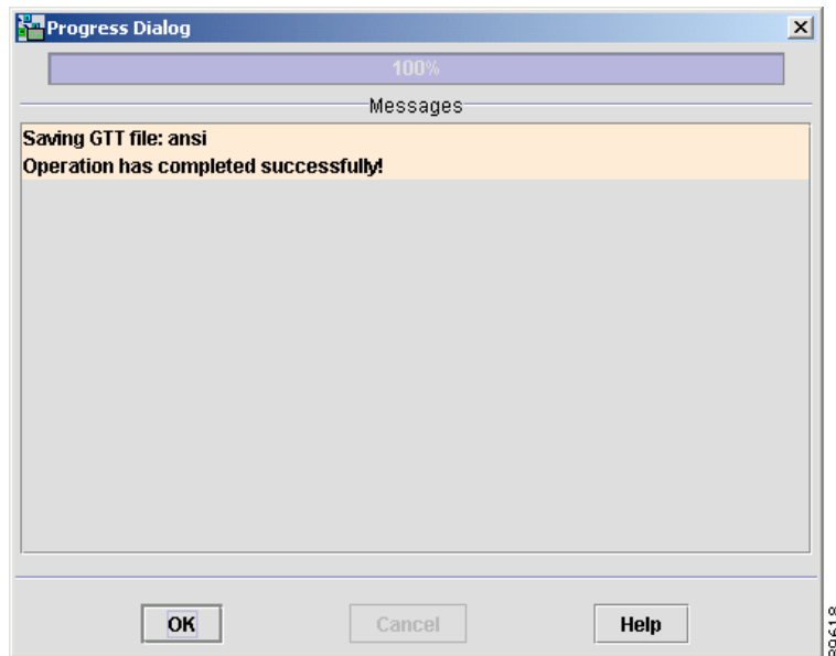
Figure 3-85 Progress Dialog
