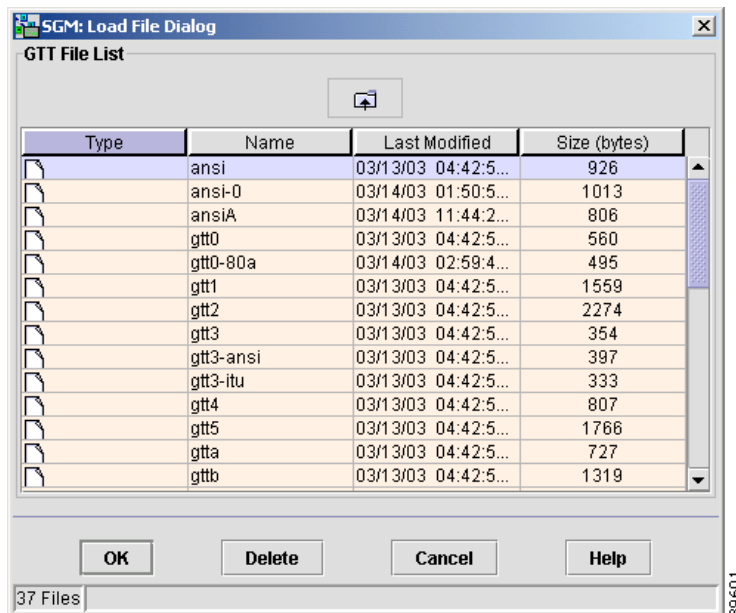
Figure 3-84 Load File Dialog: GTT File List
