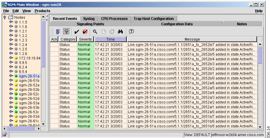
Figure 3-25 Recent Events Table for a Node
