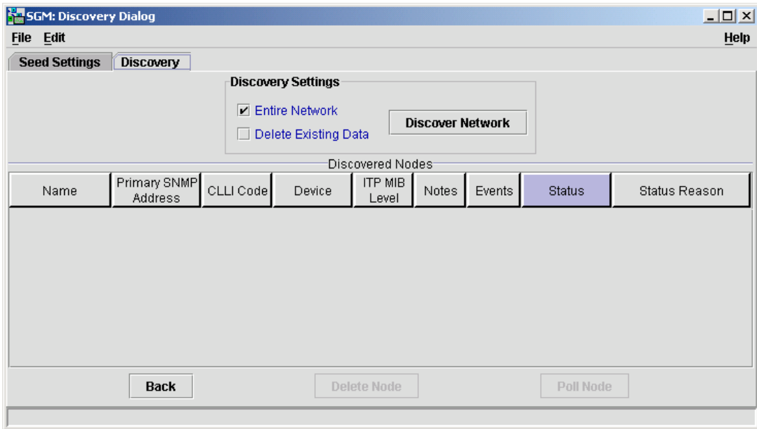
Figure 3-4 Discovery Panel
