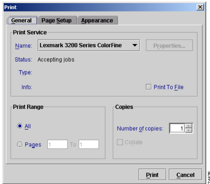
Figure 3-92 Print Dialog
