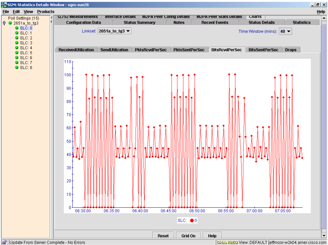
Figure 3-44 BitsRcvdPerSec Chart for a Link
