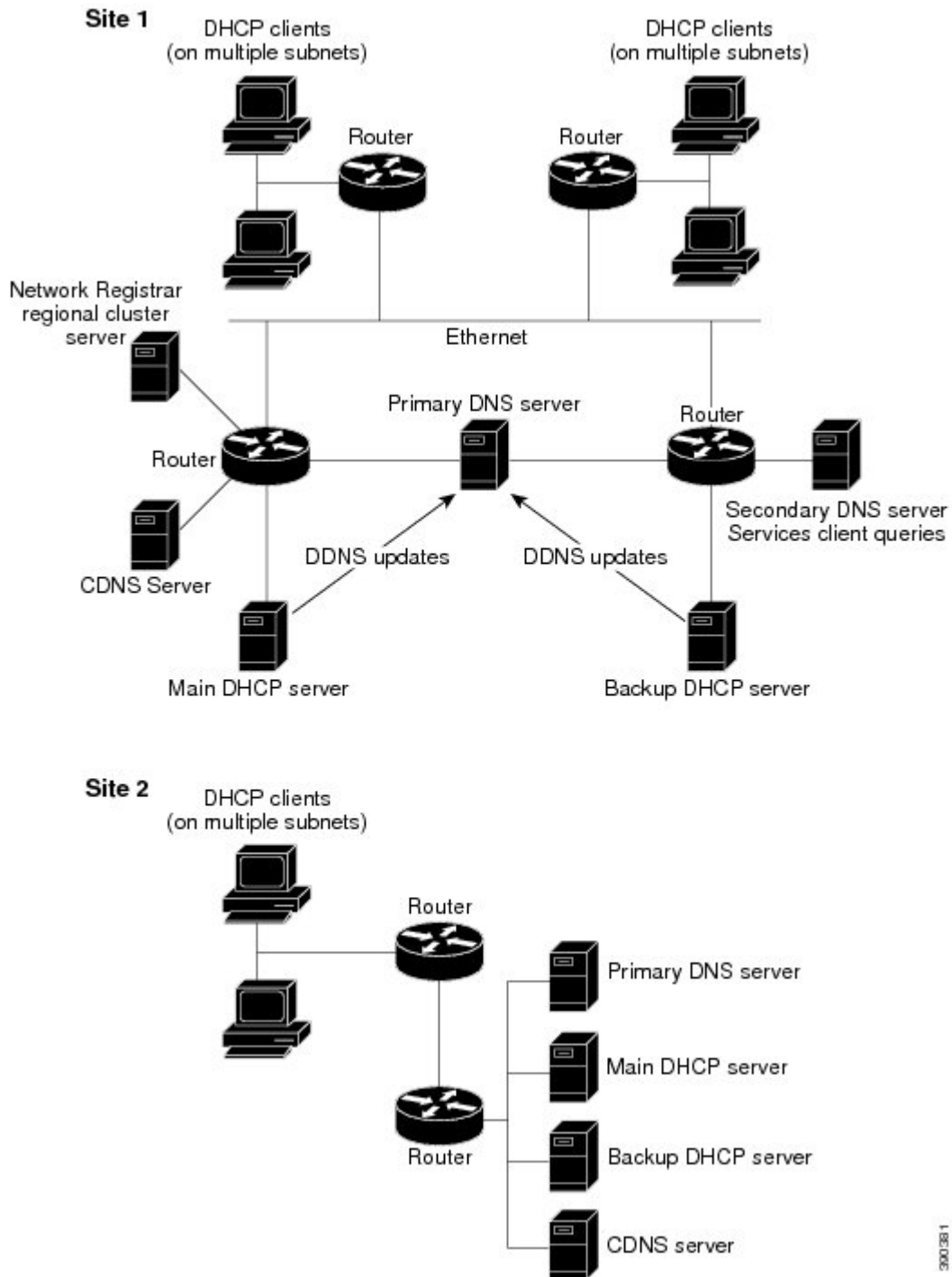
Figure 3: Large Enterprise or Service Provider Network Configuration
