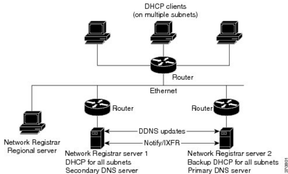
Figure 2: Small-to-Medium LAN Configuration
