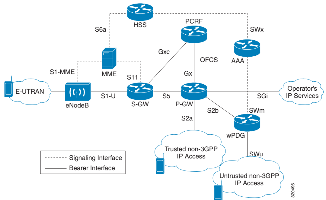
Figure 27-15 ePDG Architecture
