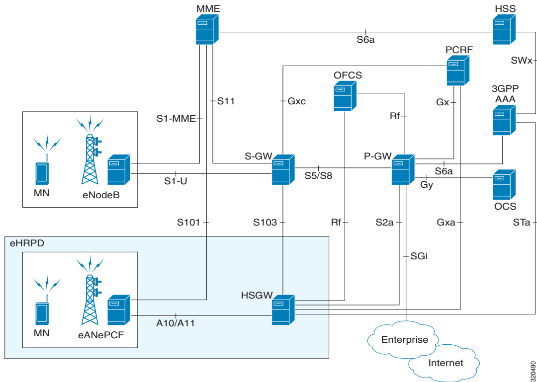
Figure 27-8 HSGW Topology
