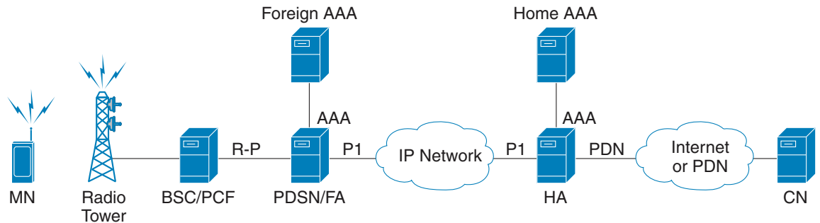
Figure 27-10 Home Agent Topology
