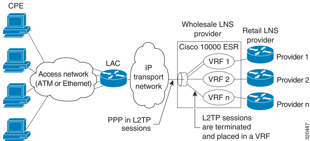
Figure 27-6 LAC Architecture
