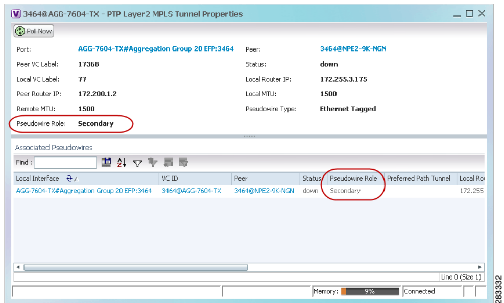
Figure 18-59 Layer 2 MPLS Tunnel Properties for Pseudowire Redundancy Service
