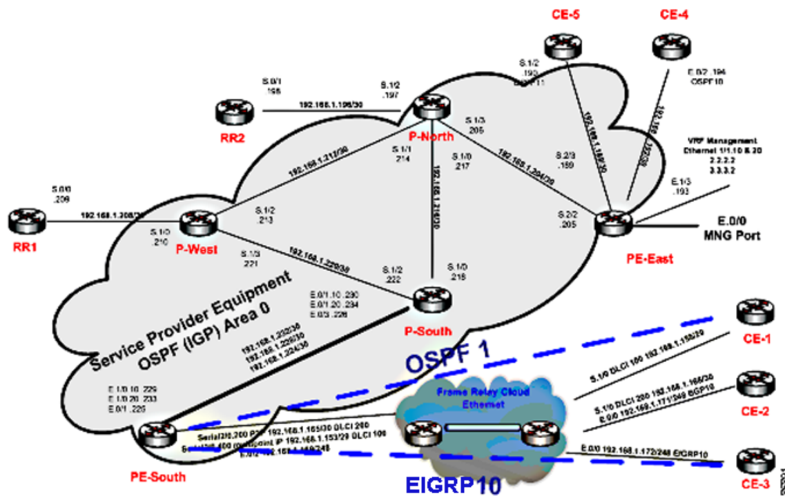
Figure C-1 Correlation Scenarios Lab Setup
