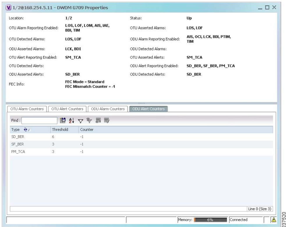
Figure 17-3 DWDM G709 Properties Window – Example 2
