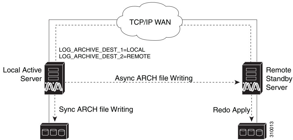
Figure 2-6 ADG Database Replication Process (ADG Geographical Redundancy)
