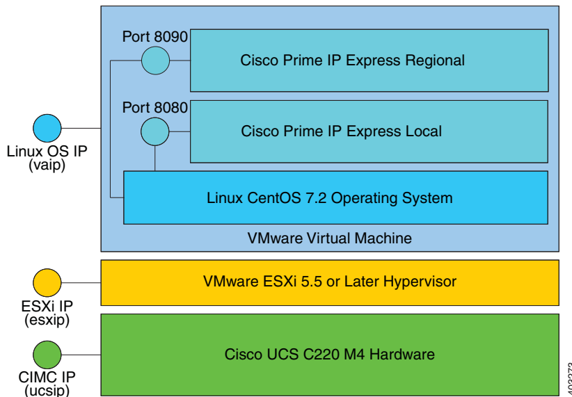
Figure 1 Cisco Prime IP Express Jumpstart Configuration
