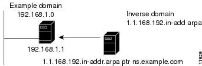
Figure 8: Reverse Domains
