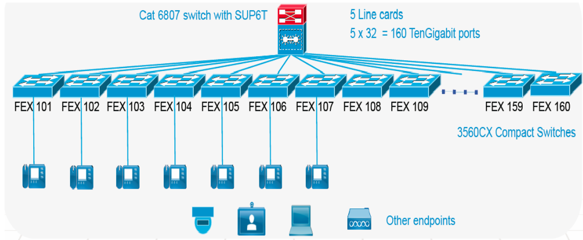
Figure 48-1 Sample Instant Access Topology
