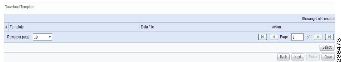
Figure 13-6 Add/Remove Templates
