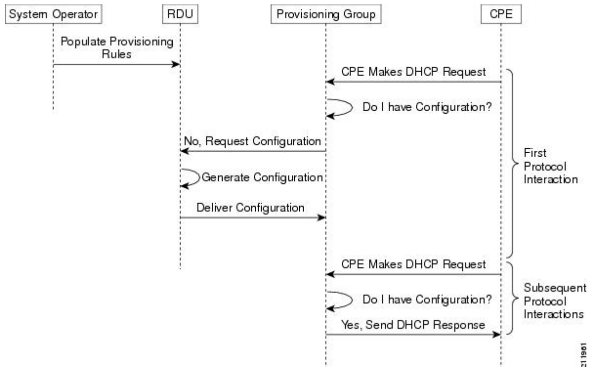
Figure 3: Workflow of Initial Device Configuration – Self-Provisioned Mode
