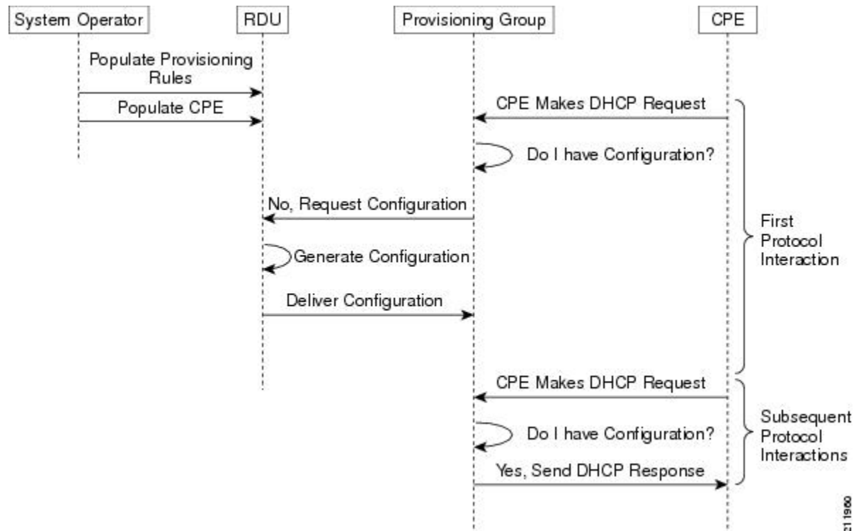
Figure 2: Workflow of Initial Device Configuration – Preprovisioned Mode
