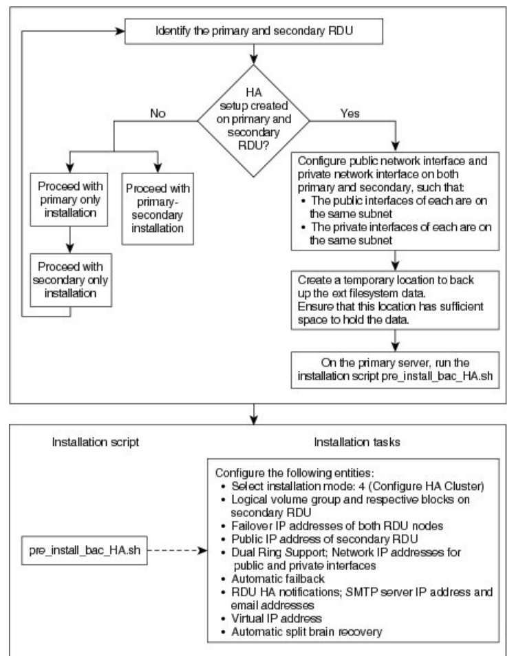
Figure 6: Configure HA Cluster
