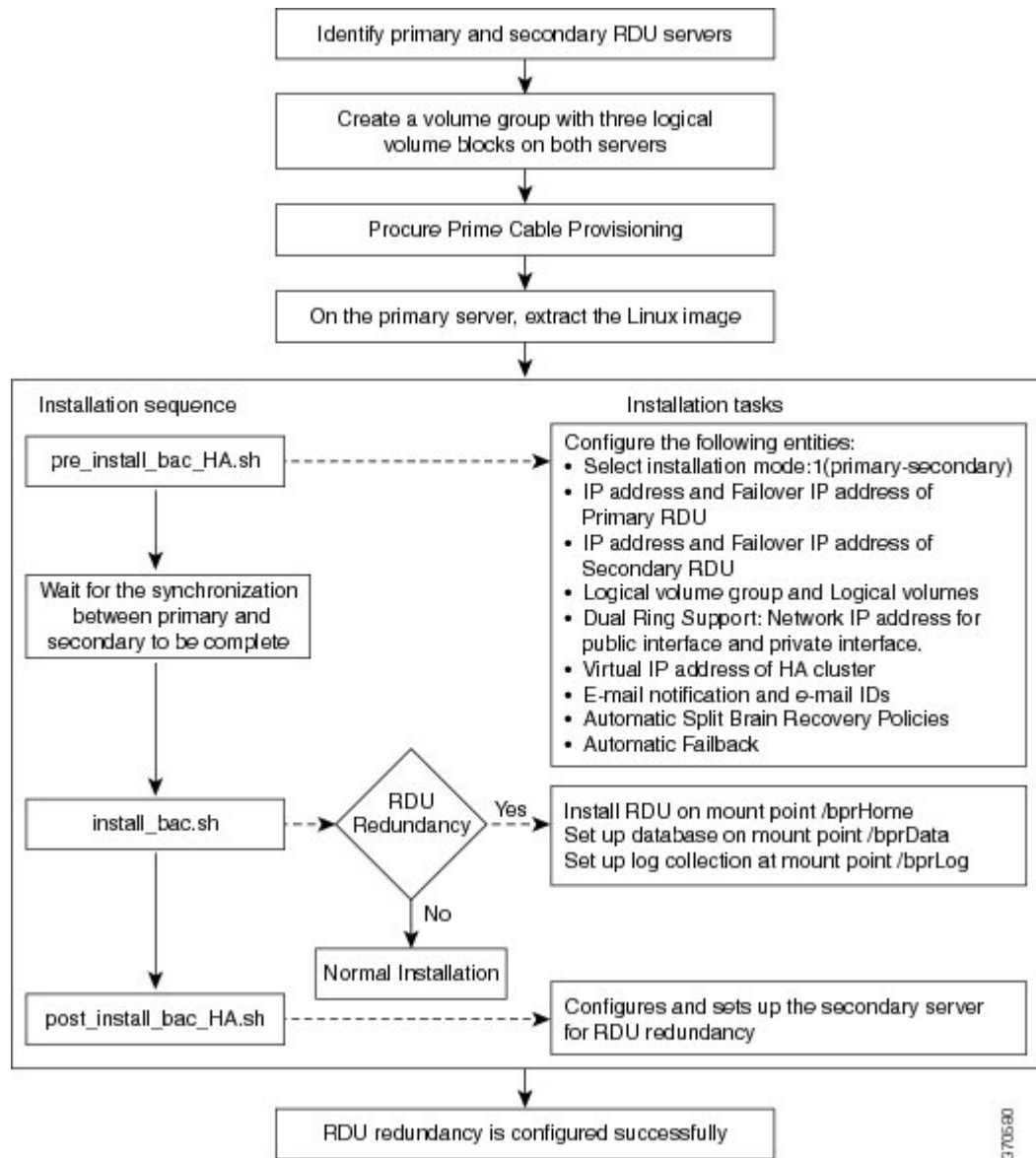
Figure 3: RDU HA Setup - primary-secondary mode
