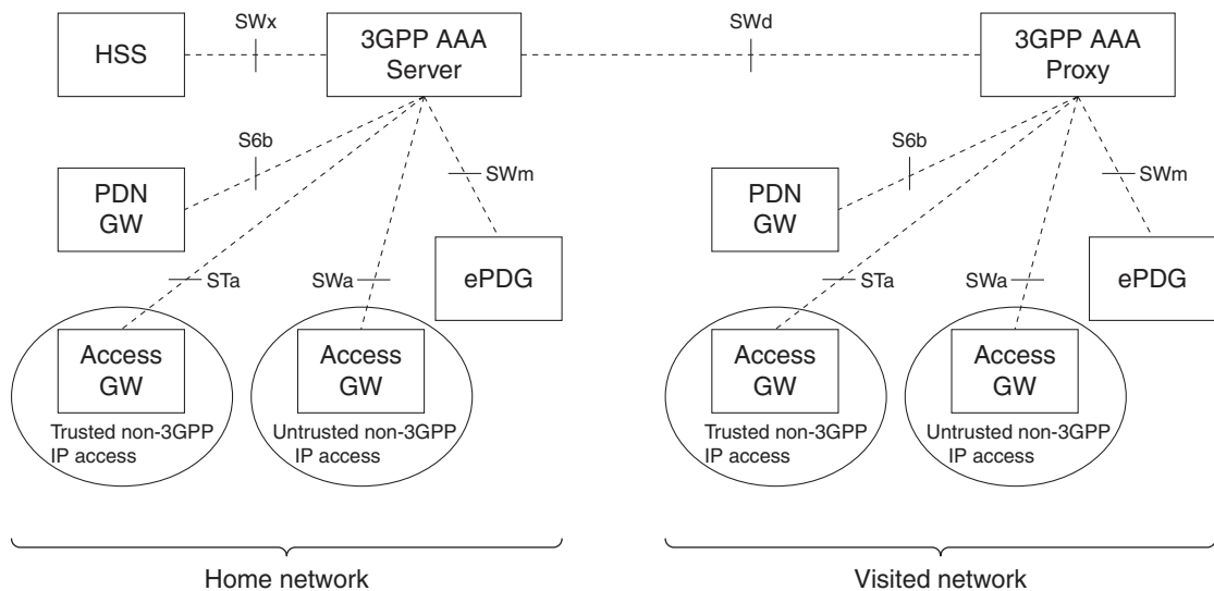
Figure 6-1 3GPP Interfaces
