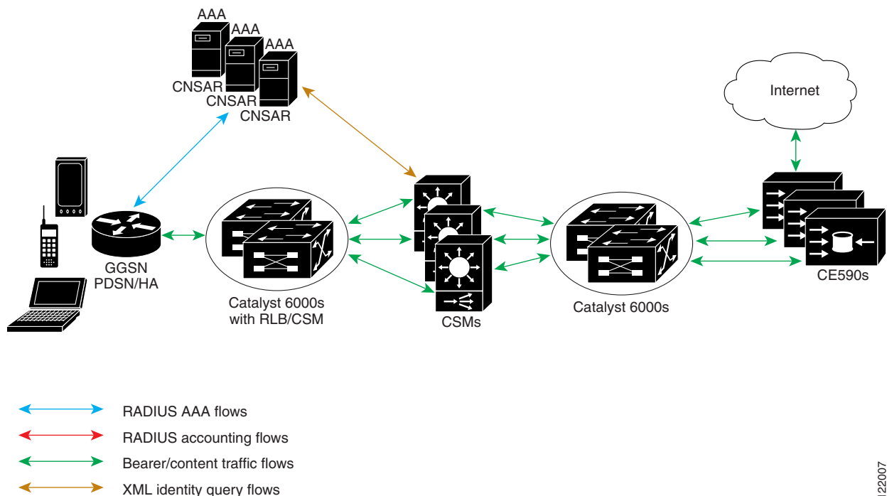
Figure 7-1 Prime Access Registrar System Overview
