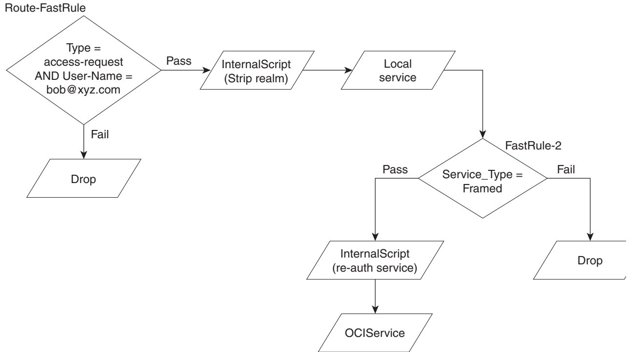
Figure 11-1 FastRules Workflow
