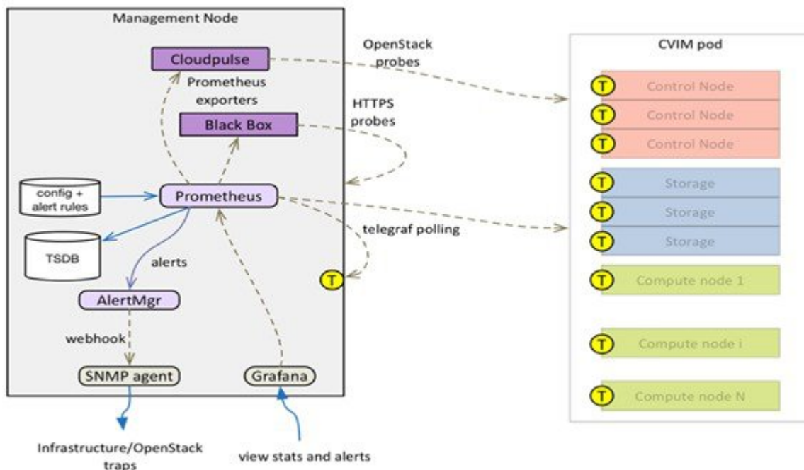
Figure 23: CVIMMON Architecture
