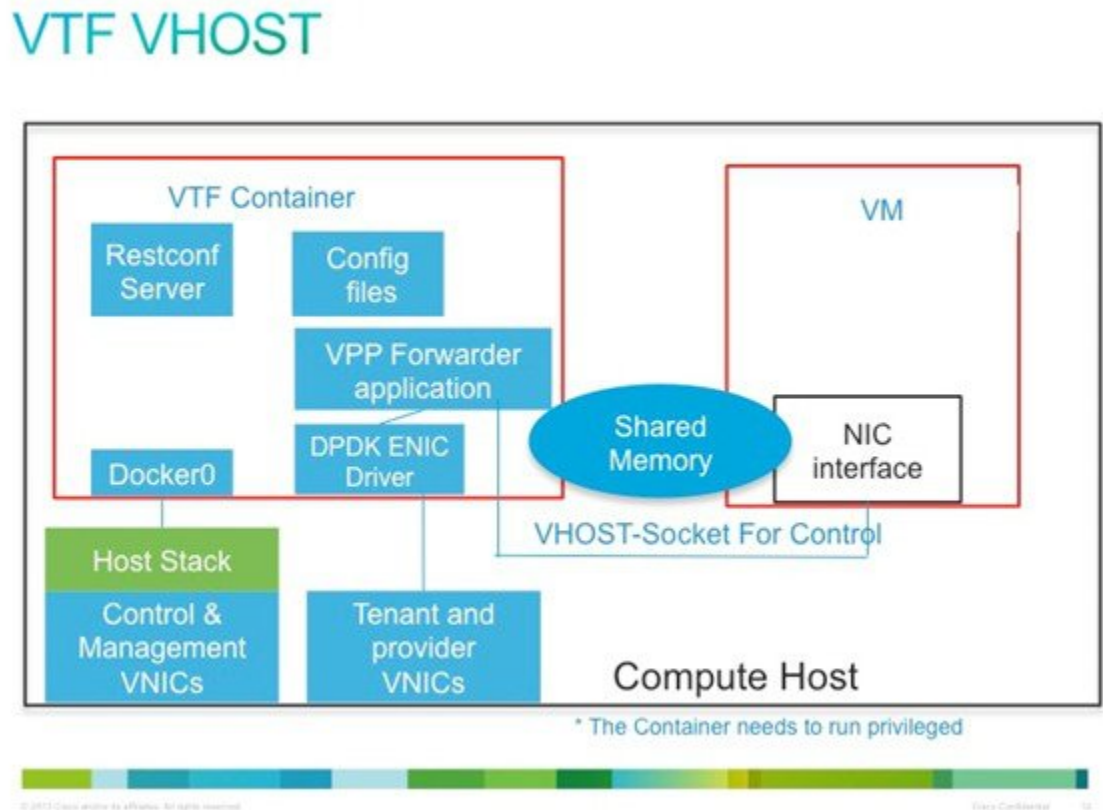
Figure 3: VTF Vhost
