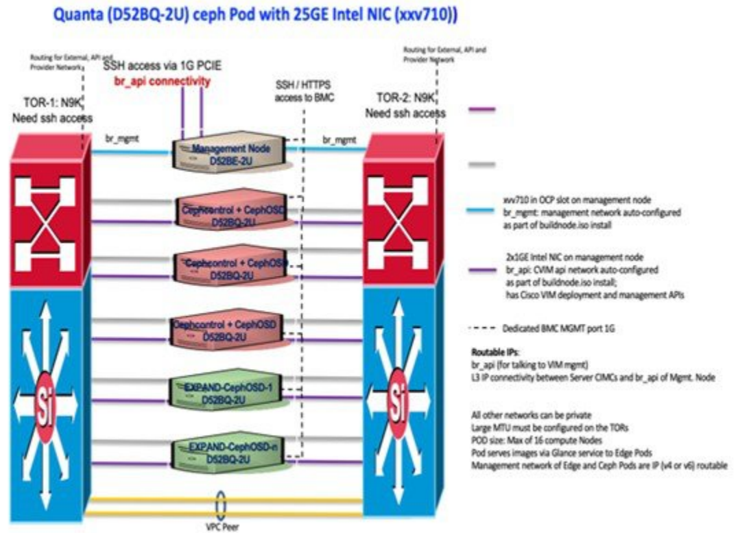
Figure 54: Quanta (D52BQ-2U) Ceph Pod with 25GE Intel NIC (xxv710)
