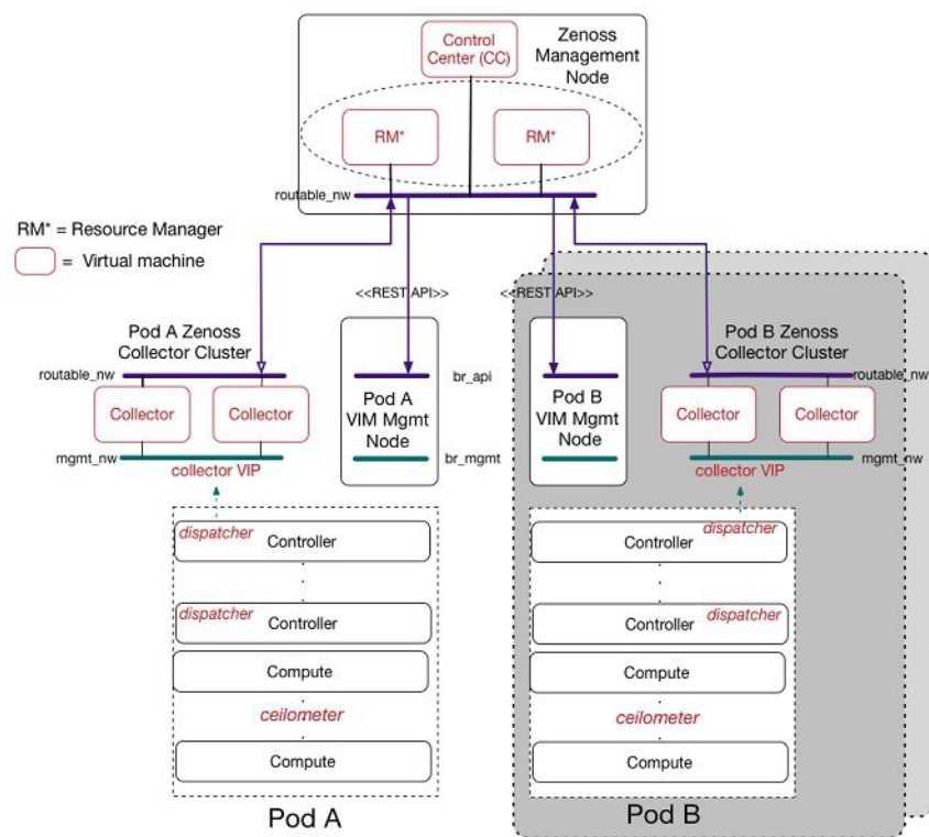
Figure 22: NFVIMON Architecture
