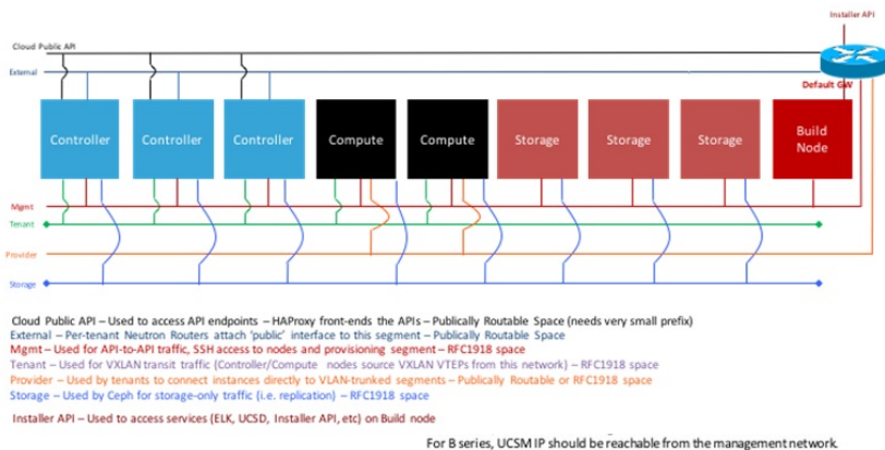
Figure 18: Network and VLAN Layout for Combined C-Series and B-Series Installation
