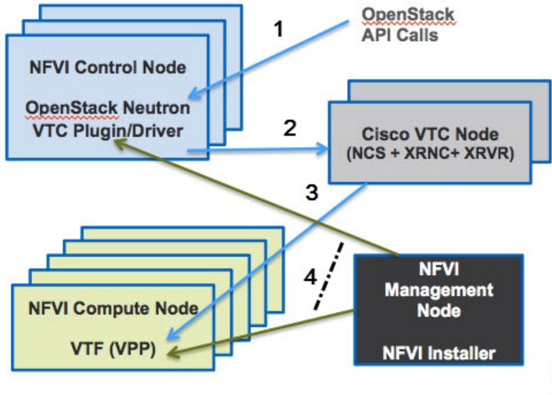
Figure 20: Cisco VTS in Cisco NFVI
