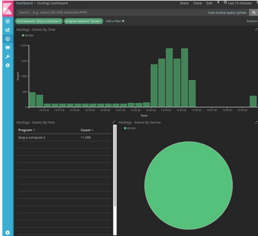
Figure 6: Hostlogs Dashboard
