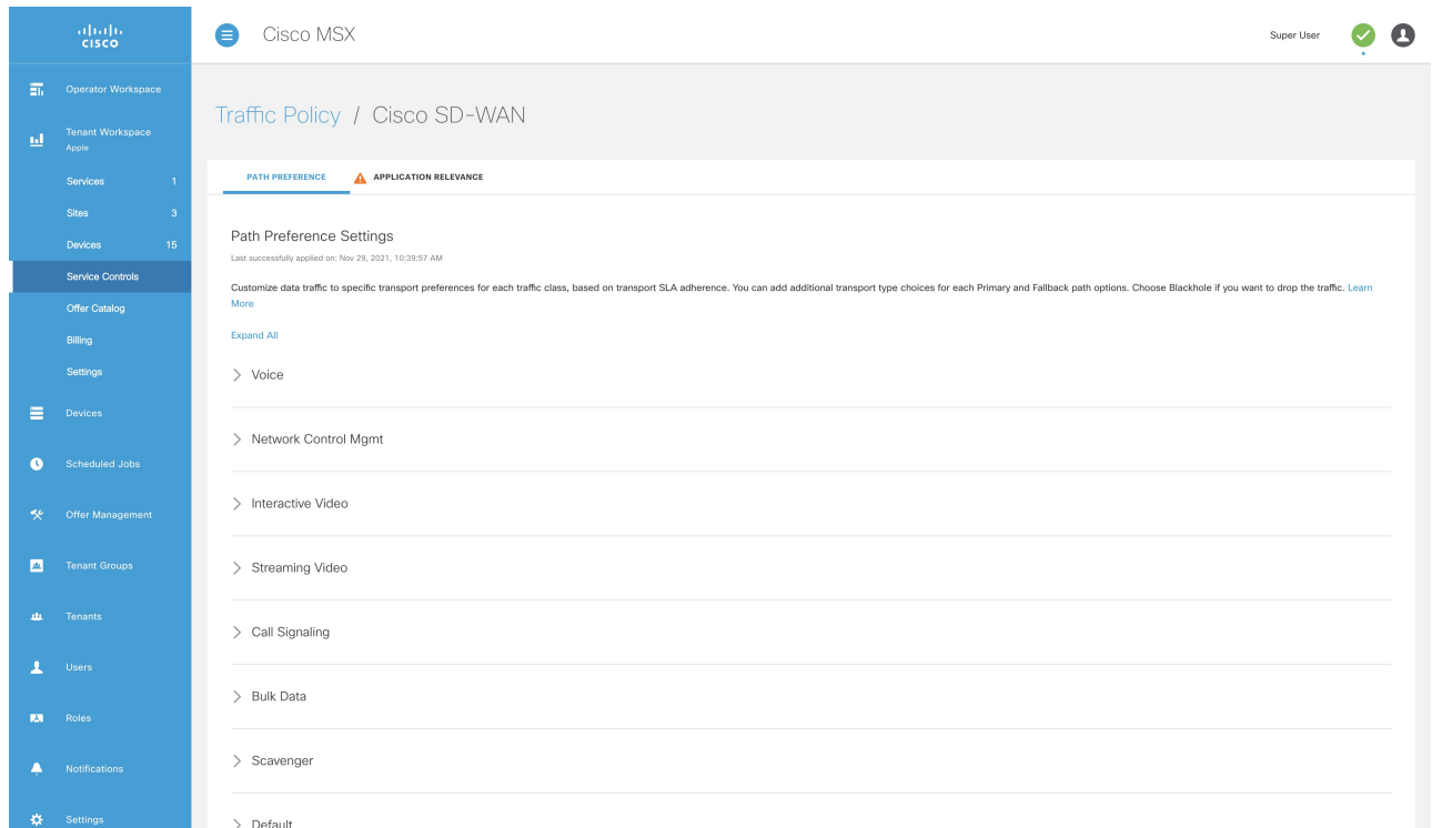
Figure 13: Configuring Path Preference
