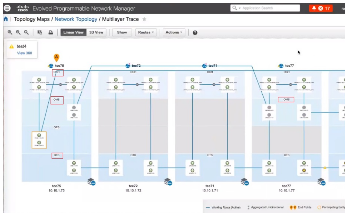
Figure 1: Multilayer Trace View
