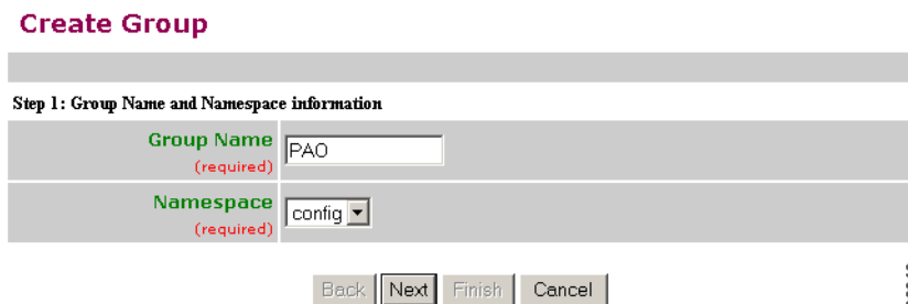
Figure 6-2 Create Group
