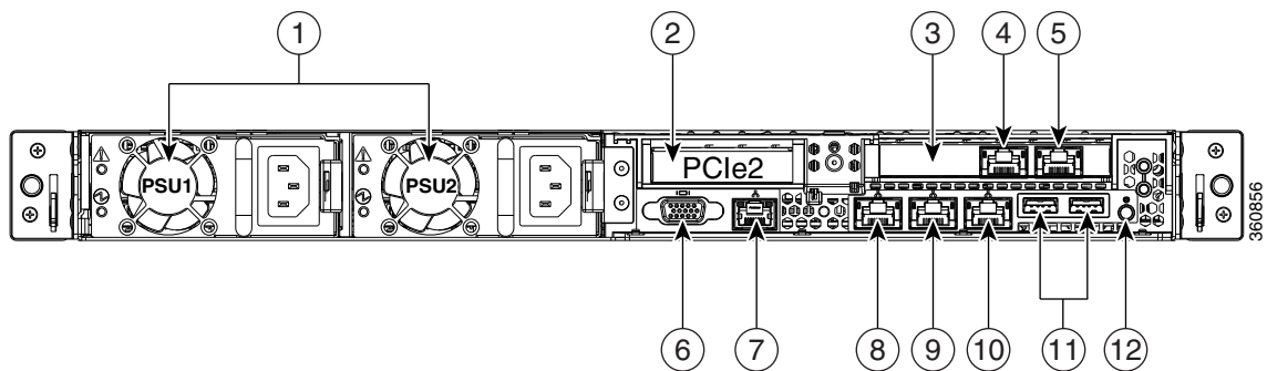
Figure 2 Cisco SNS-3415/3495 Appliance Rear View
