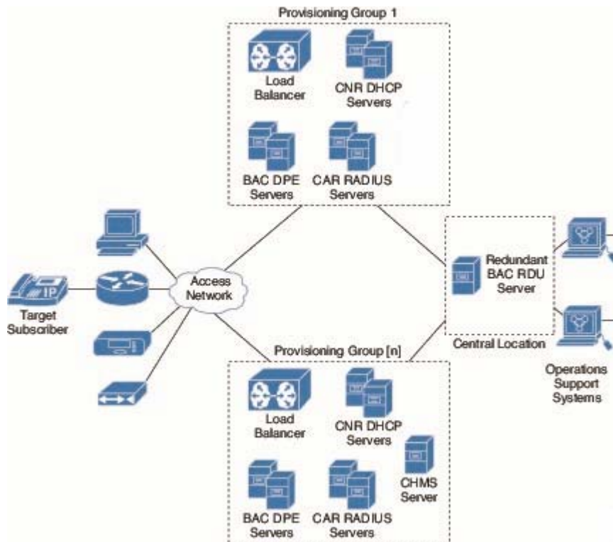
Figure 2-1 CWMP Deployment in Cisco BAC
