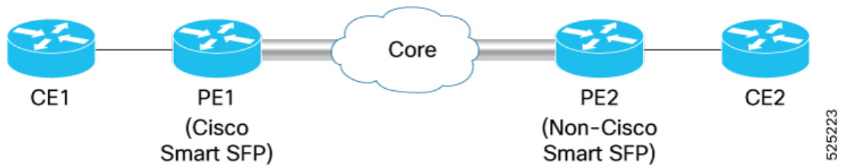
Figure 1: Packet transmission using Cisco Smart SFP with destination MAC address
