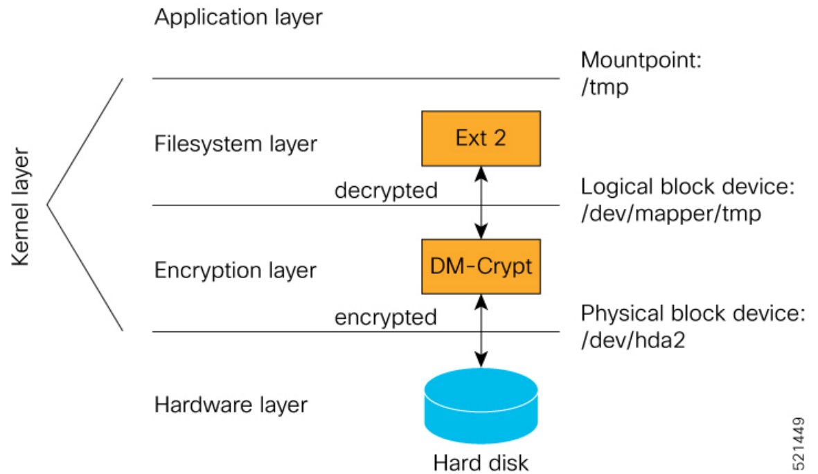
Figure 21: DM-Crypt Encryption
