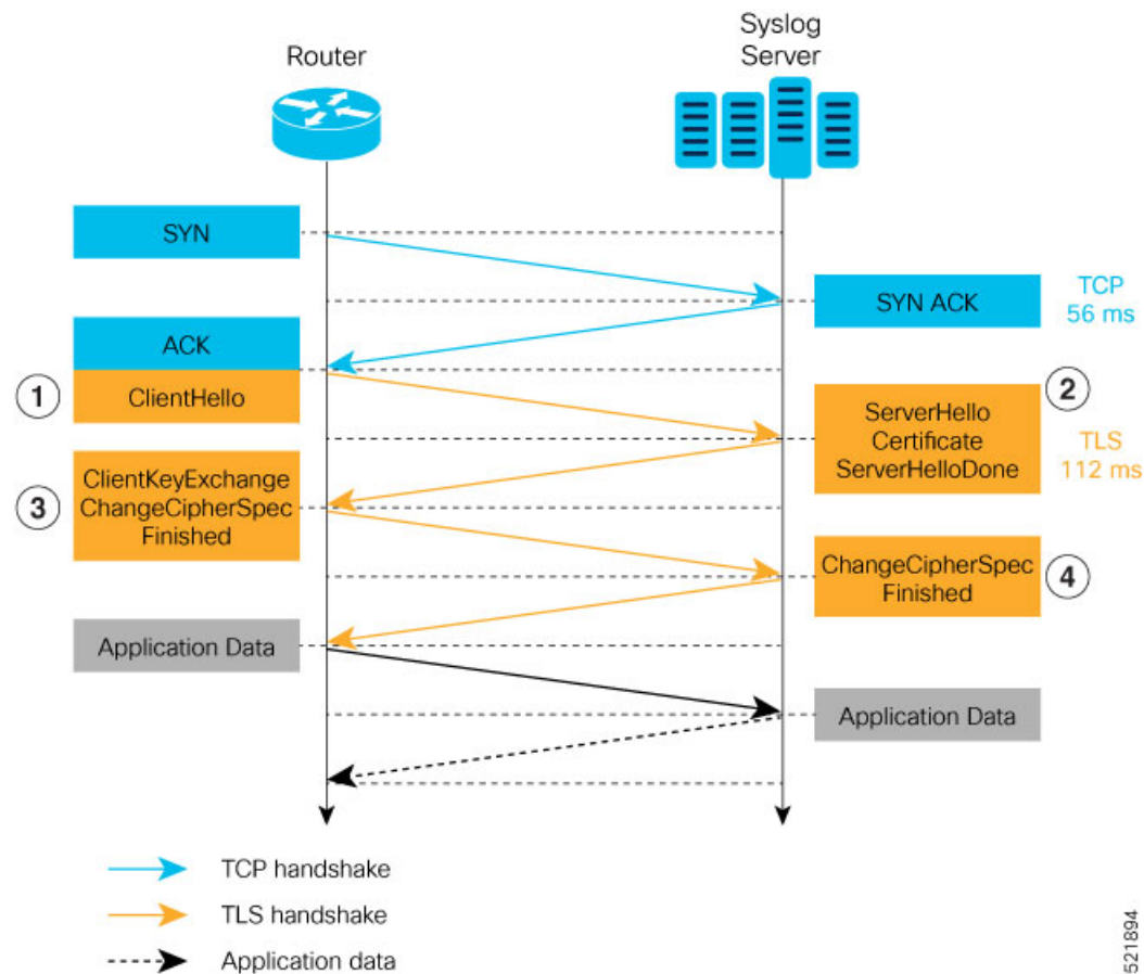
Figure 10: TLS Handshake
