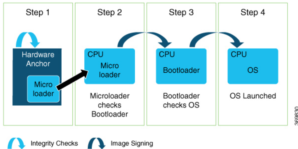
Figure 19: Secure Boot
