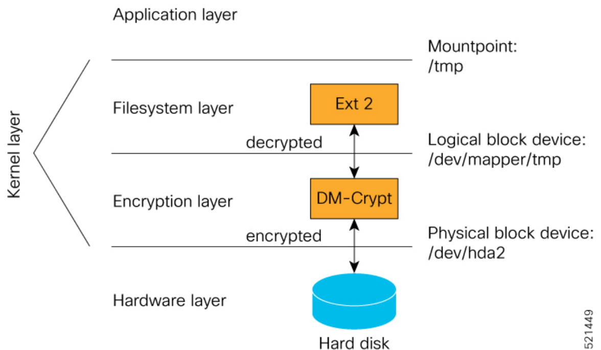
Figure 12: DM-Crypt Encryption
