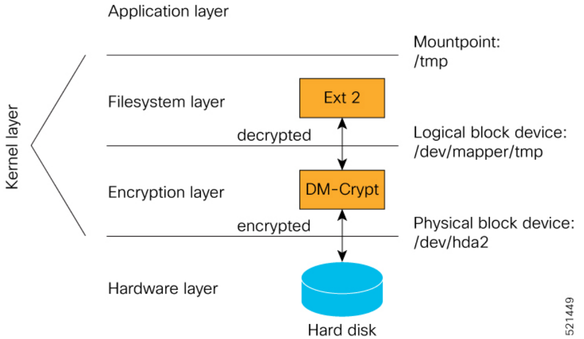
Figure 12: DM-Crypt Encryption
