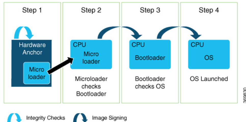
Figure 11: Secure Boot
