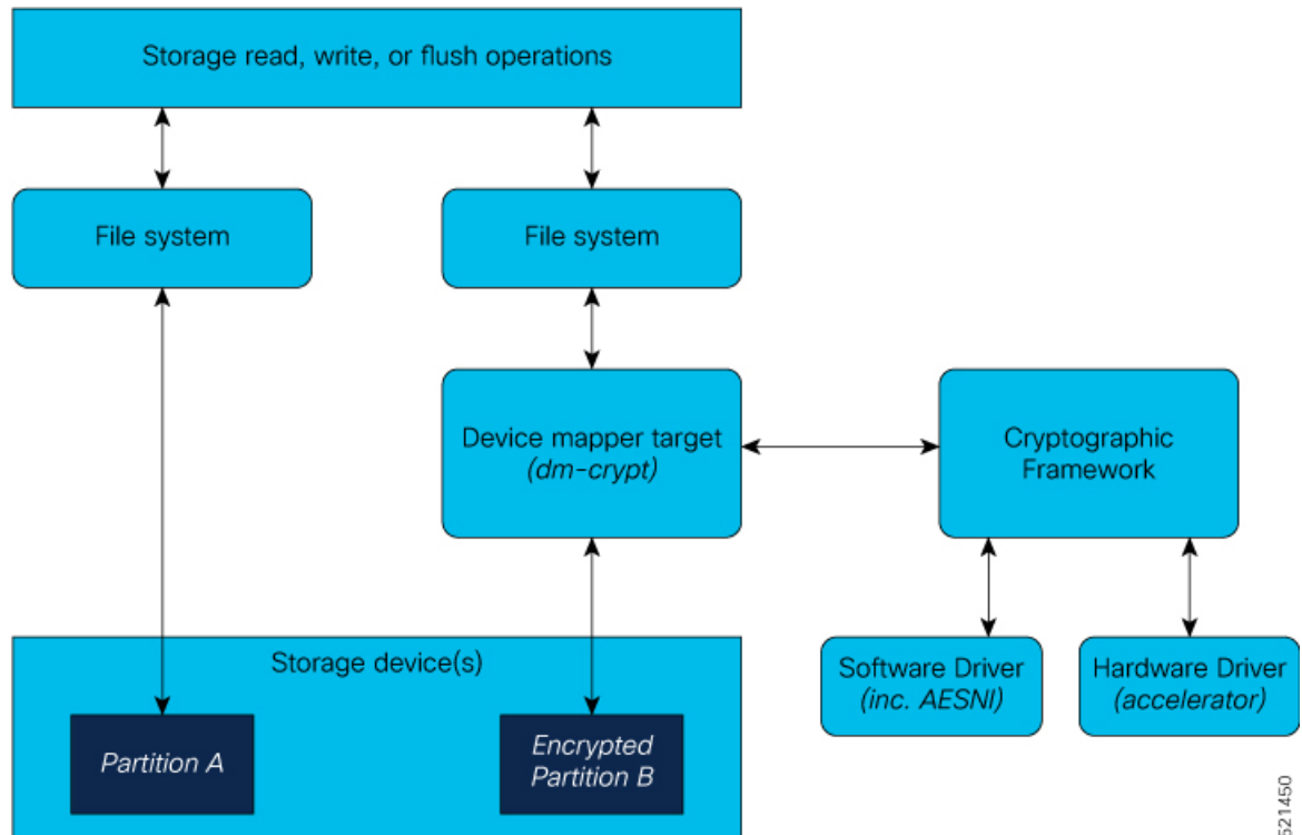
Figure 11: AES-NI Support
