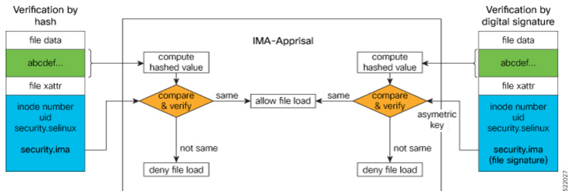
Figure 12: IMA Appraisal
