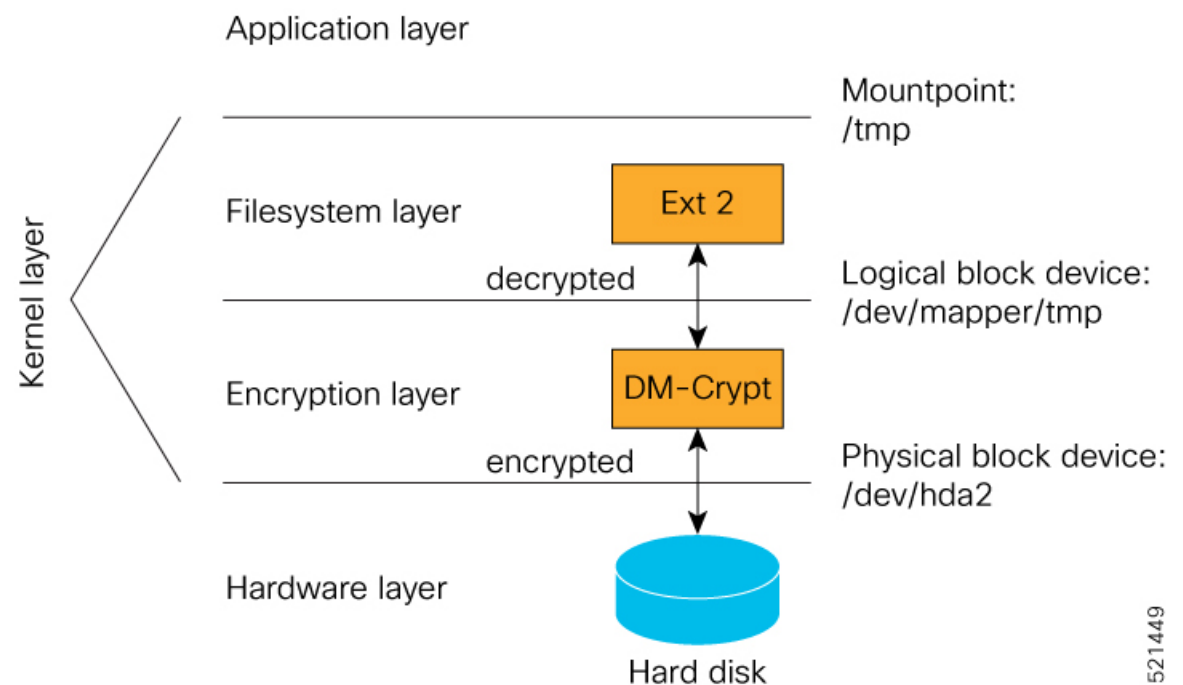
Figure 23: DM-Crypt Encryption
