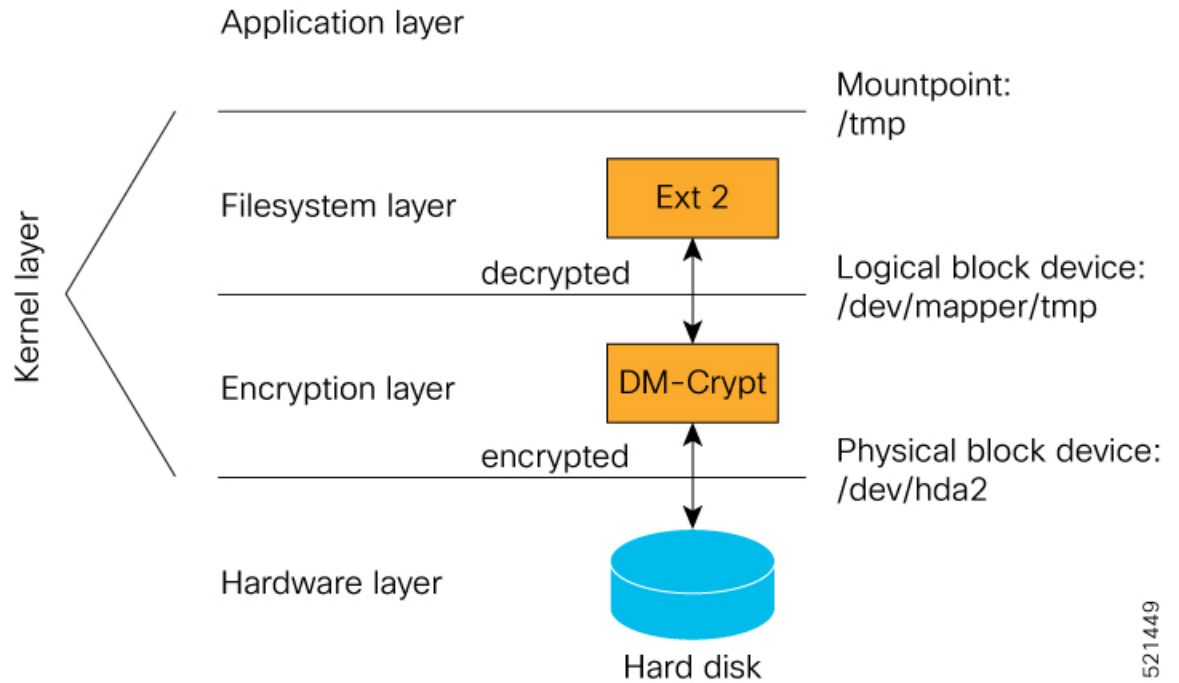
Figure 22: DM-Crypt Encryption
