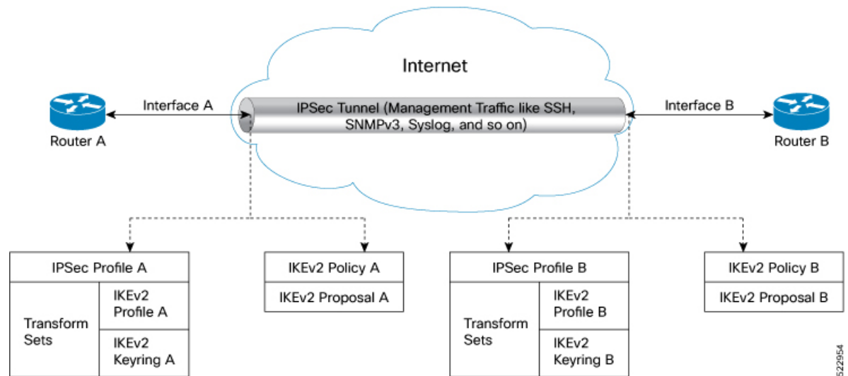
Figure 9: IPsec for Management Traffic Flow Between Two Routers
