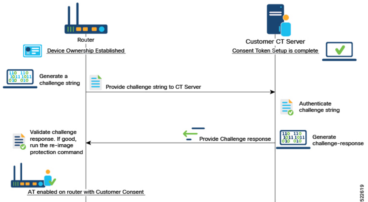
Figure 18: Workflow for the Customer Consent Token Key
