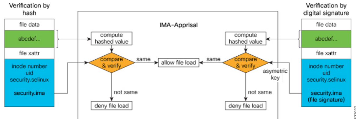
Figure 24: IMA Appraisal
