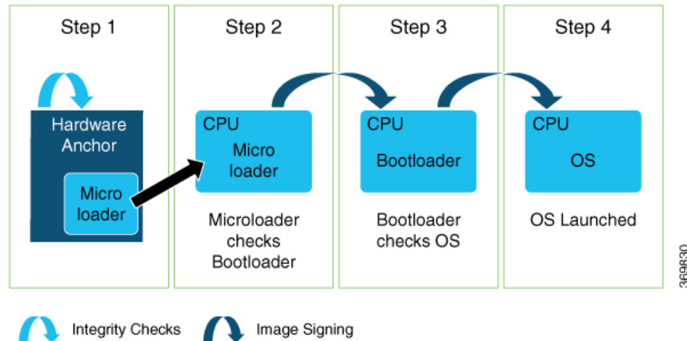
Figure 21: Secure Boot
