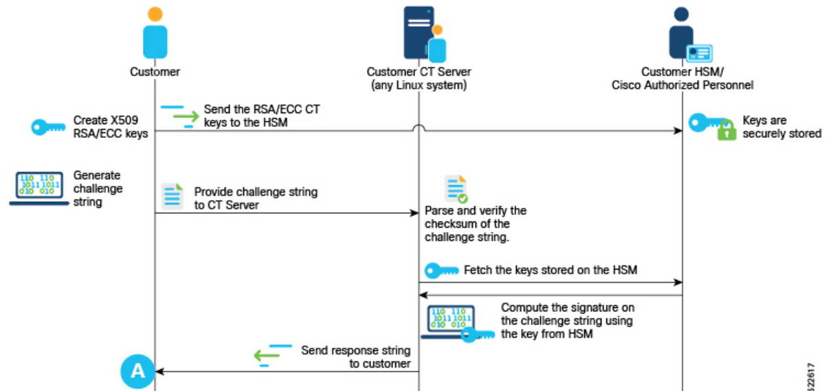
Figure 1: Workflow for the Consent Token Server
