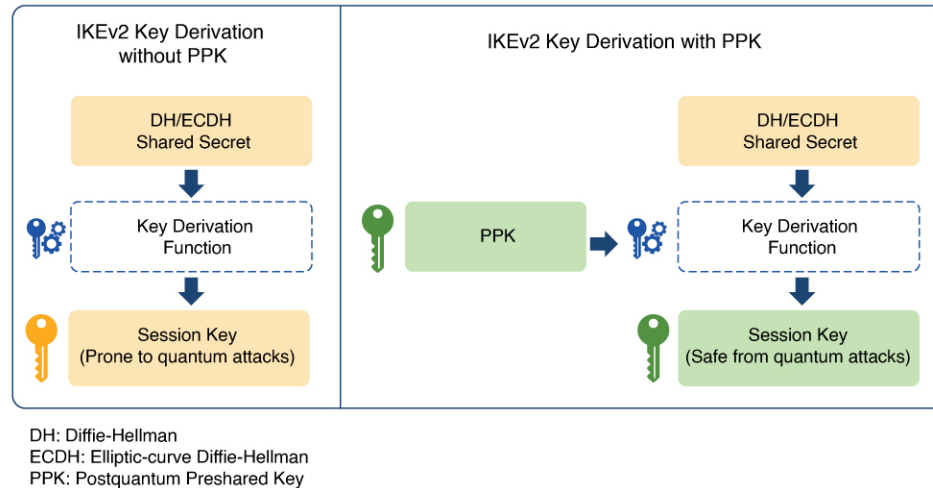
Figure 2: IKEv2 Key Derivation - With and Without PPK
