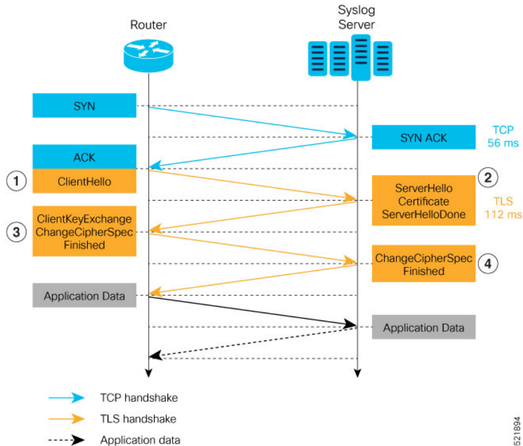
Figure 1: TLS Handshake
