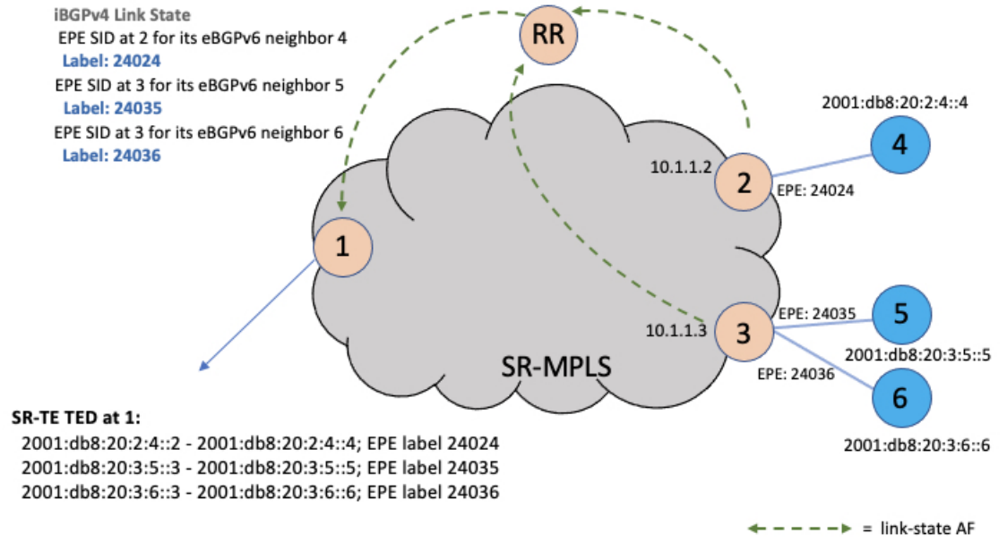
Figure 7: BGP-LS
