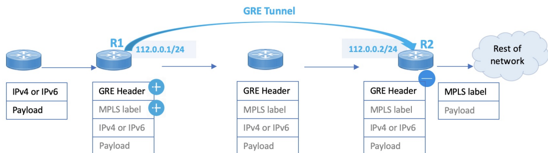
Figure 1: MPLS Over a Single-Pass GRE Tunnel
