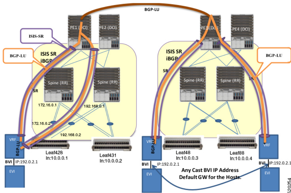
Figure 11: EVPN Bridging and VPWS Services over BGP-LU Underlay
