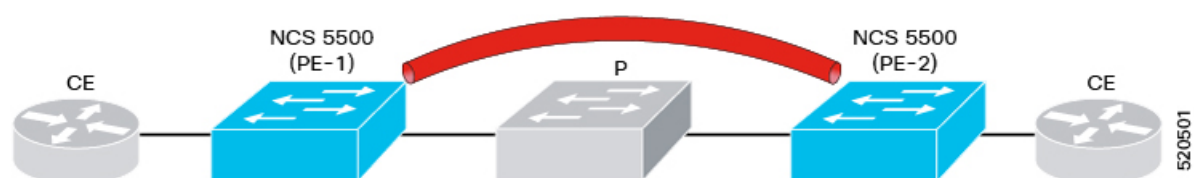
Figure 3: L2CP Tunneling
