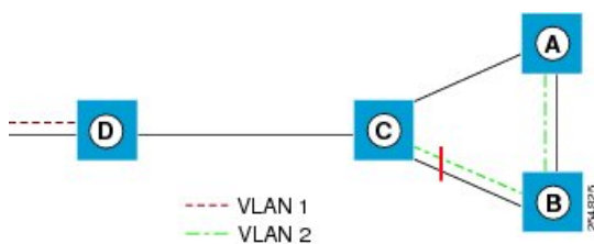
Figure 31: Flush Containment
