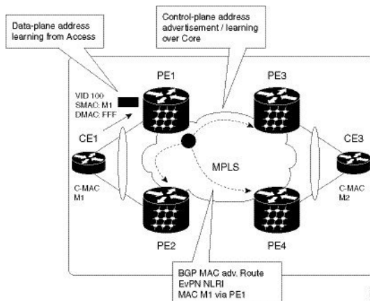
Figure 41: EVPN Operation
