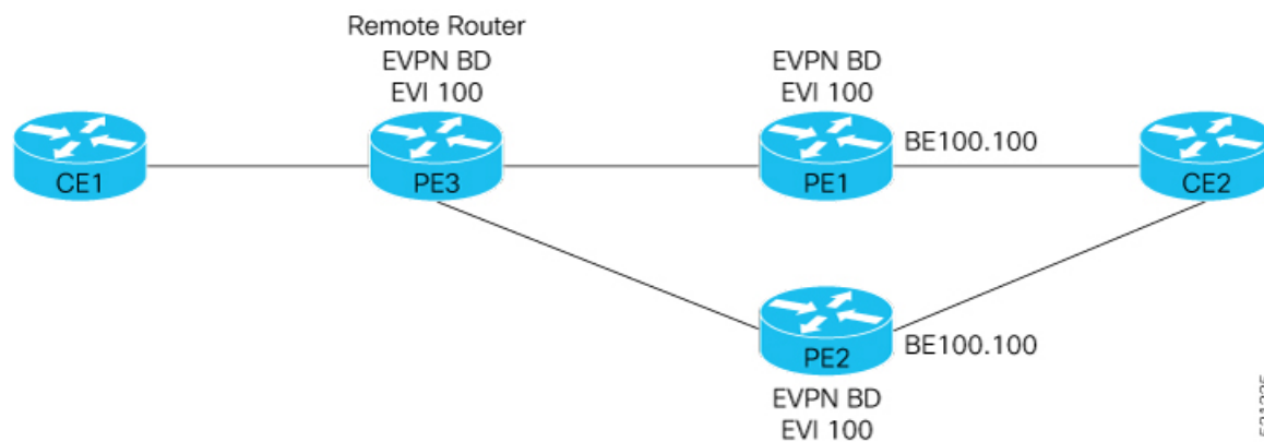
Figure 52: Layer 2 Fast Reroute
