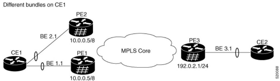
Figure 57: EVPN: Single-Active Multihoming for Anycast Gateway IRB
