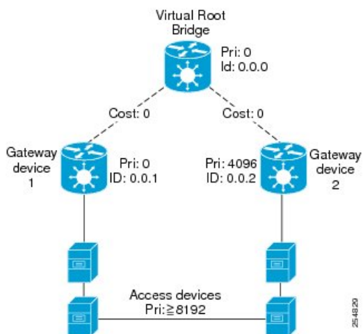
Figure 36: MSTAG Guidelines
