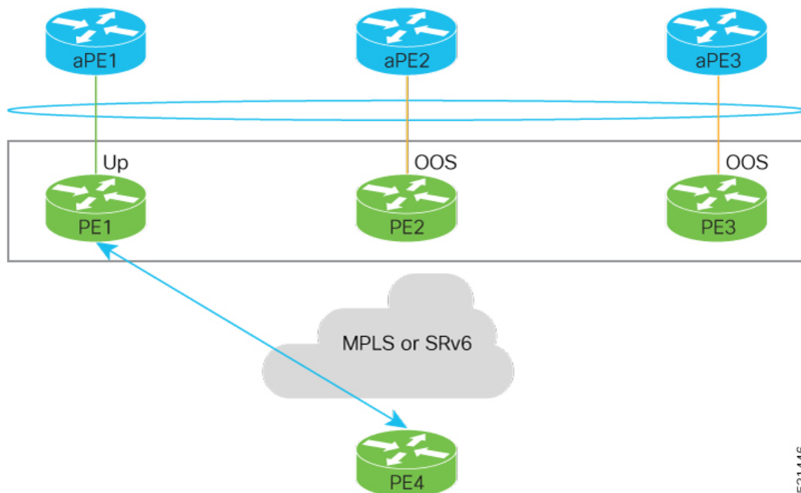
Figure 53: EVPN Access-Driven DF Election
