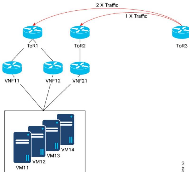
Figure 15: Proportional Multipath
