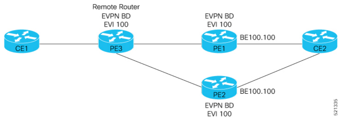
Figure 17: Layer 2 Fast Reroute
