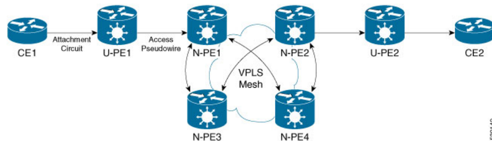
Figure 1: Access Pseudowire
