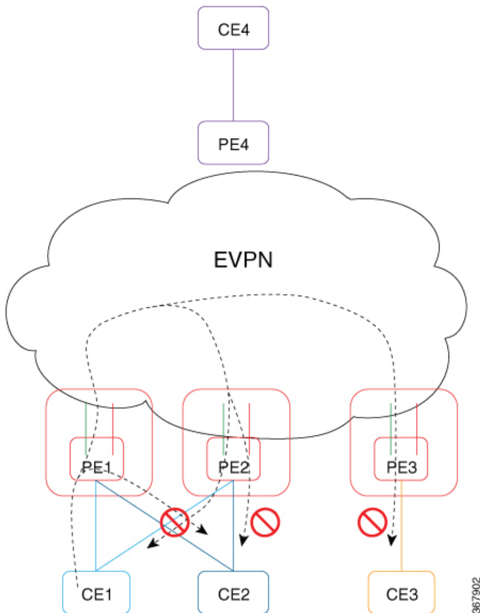
Figure 4: EVPN E-Tree
