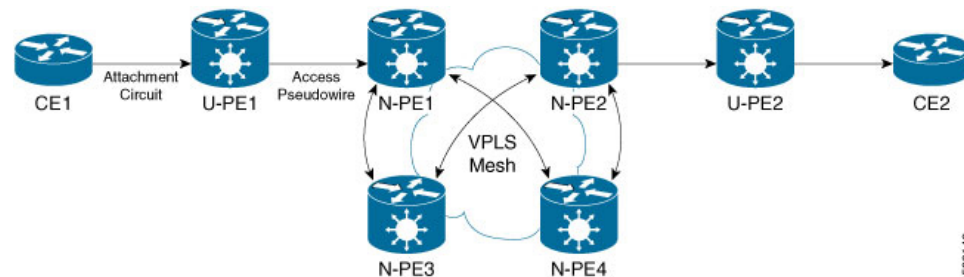
Figure 1: Access Pseudowire
