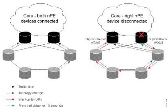
Figure 40: Active Topology Change
