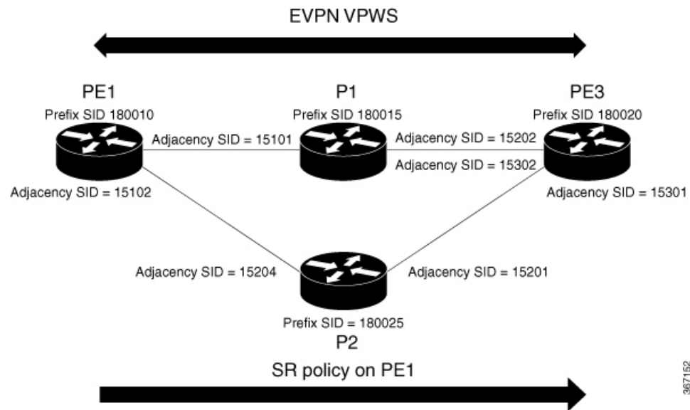
Figure 77: EVPN VPWS Preferred Path over SR-TE Policy
