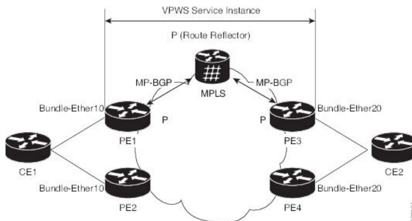
Figure 59: Layer 2 FRR multi-homing topology
