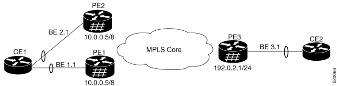
Figure 64: EVPN: Single-Active Multihoming for Anycast Gateway IRB
