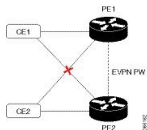
Figure 13: Local Switching
