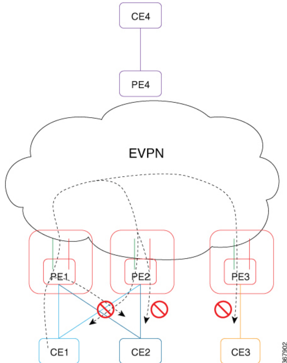
Figure 67: EVPN E-Tree
