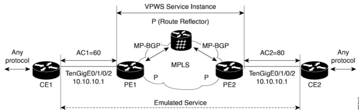
Figure 76: VPWS Traffic flow
