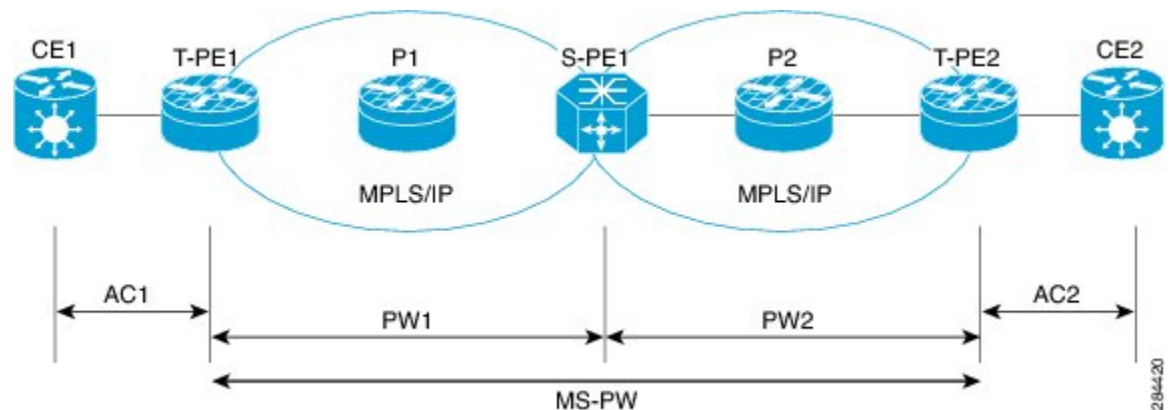
Figure 14: Multisegment Pseudowire
