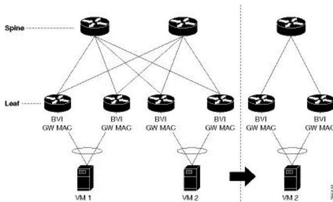
Figure 61: EVPN IRB
