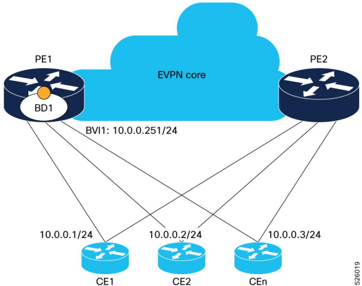
Figure 72: A sample topology for L3 EVPN IGMP and MLD state synchronization
