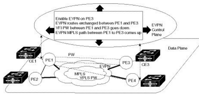
Figure 48: EVPN MPLS Seamless Integration with VPLS
