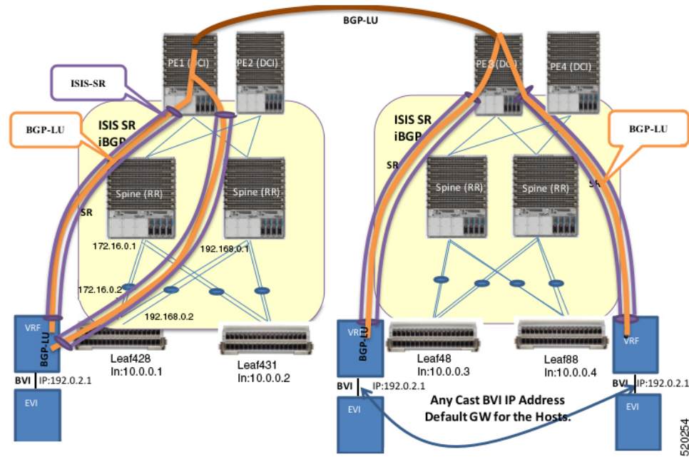
Figure 55: EVPN Bridging and VPWS Services over BGP-LU Underlay
