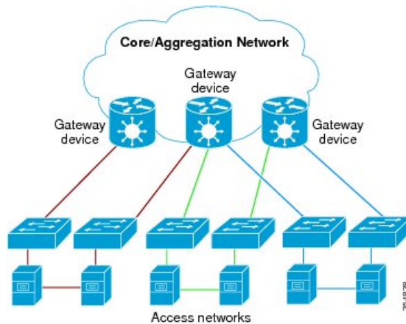
Figure 35: Access Networks
