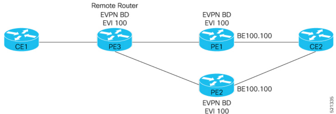
Figure 59: Layer 2 FRR multi-homing topology
