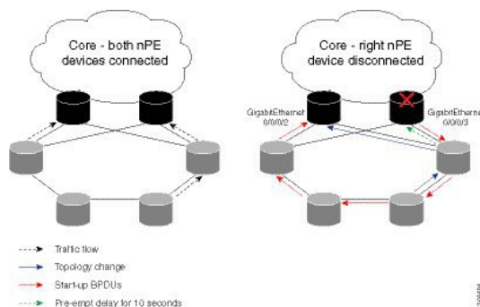
Figure 40: Active Topology Change
