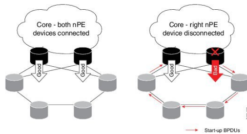
Figure 39: Core connectivity Failure
