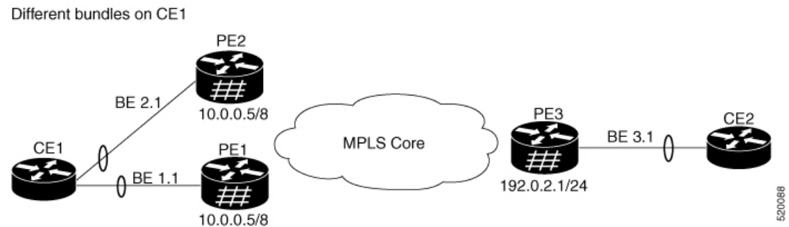
Figure 64: EVPN: Single-Active Multihoming for Anycast Gateway IRB
