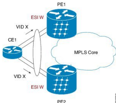
Figure 45: Dual Home Device —All-Active Load Balancing Mode
