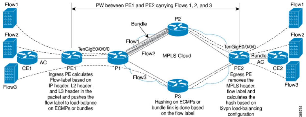
Figure 74: FAT PW with Two Flows Distributing over ECMPs and Bundle
