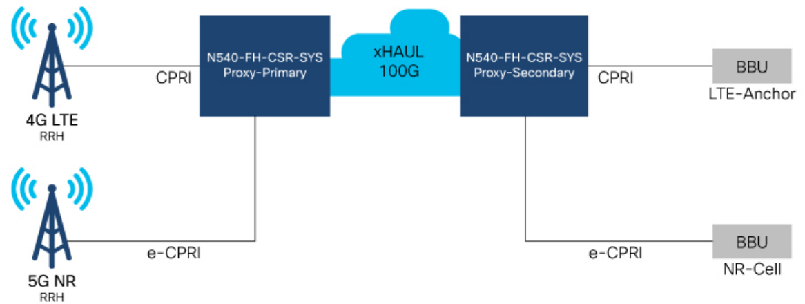
Figure 72: EVPN-VPWS to RoE Interface
