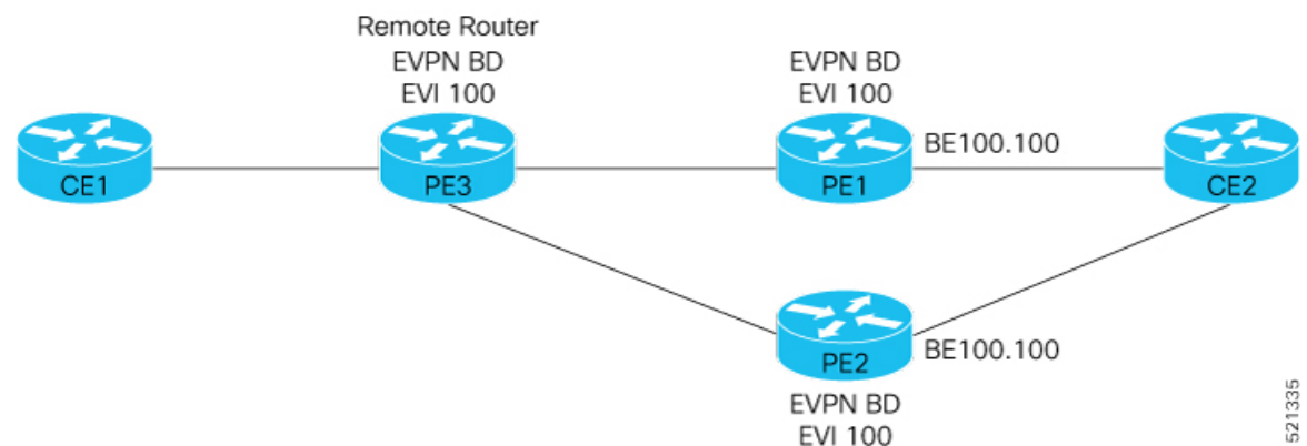
Figure 58: Layer 2 Fast Reroute
