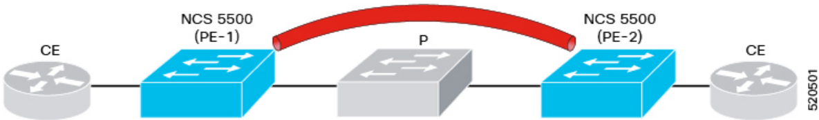
Figure 3: L2CP Tunneling
