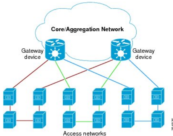
Figure 33: Core or Aggregation Network
