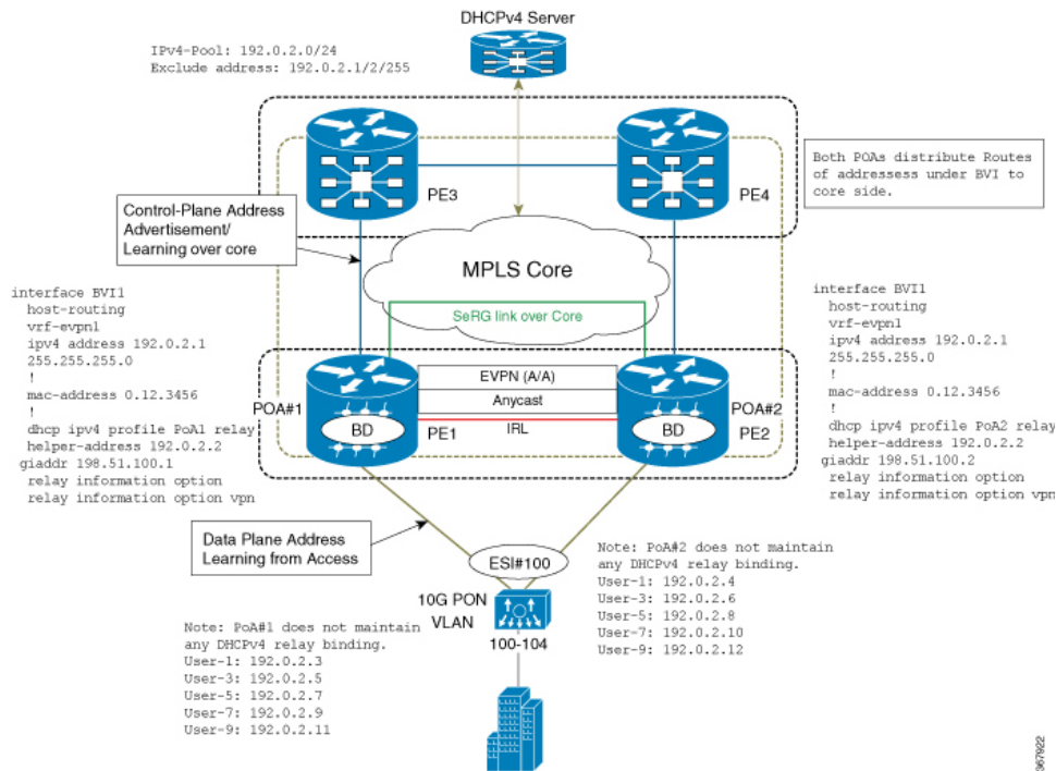
Figure 70: DHCPv4 Relay Handling for EVPN and DHCPv4 Server in Different VRF
