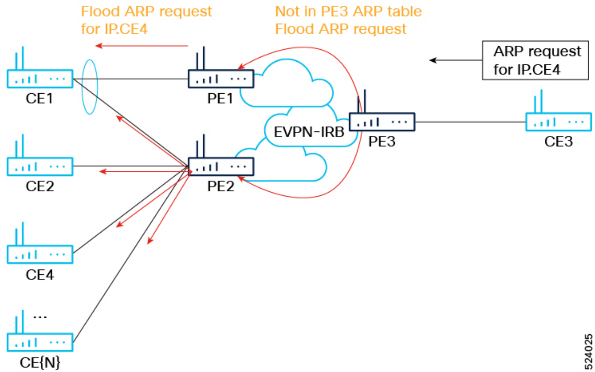
Figure 65: EVPN-IRB Network without ARP and ND Proxy Full Suppression or with ARP Proxy Partial Suppression
