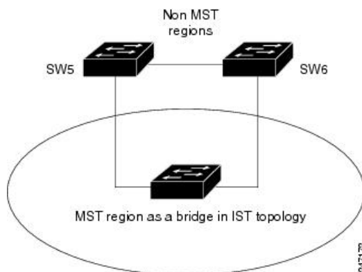
Figure 31: Logical Topology in MST Region Interacting with Non-MST Bridges
