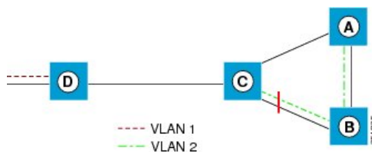
Figure 32: Flush Containment
