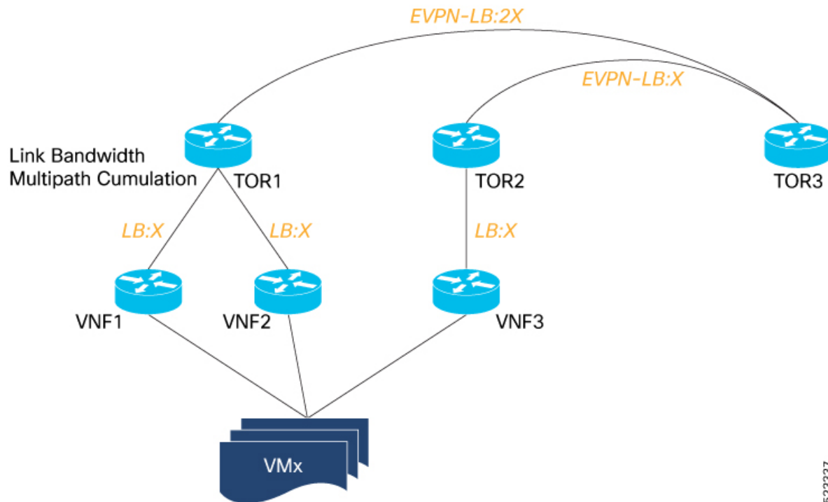
Figure 57: EVPN Link Bandwidth
