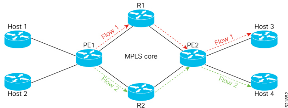
Figure 29: Fat label-based load balancing on L2VPN decapsulation node workflow
