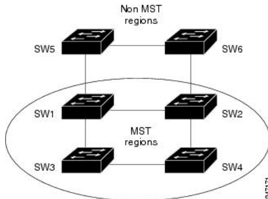
Figure 30: MST Interaction with Non-MST Regions
