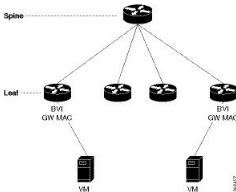
Figure 62: EVPN Single-Homing Access Gateway
