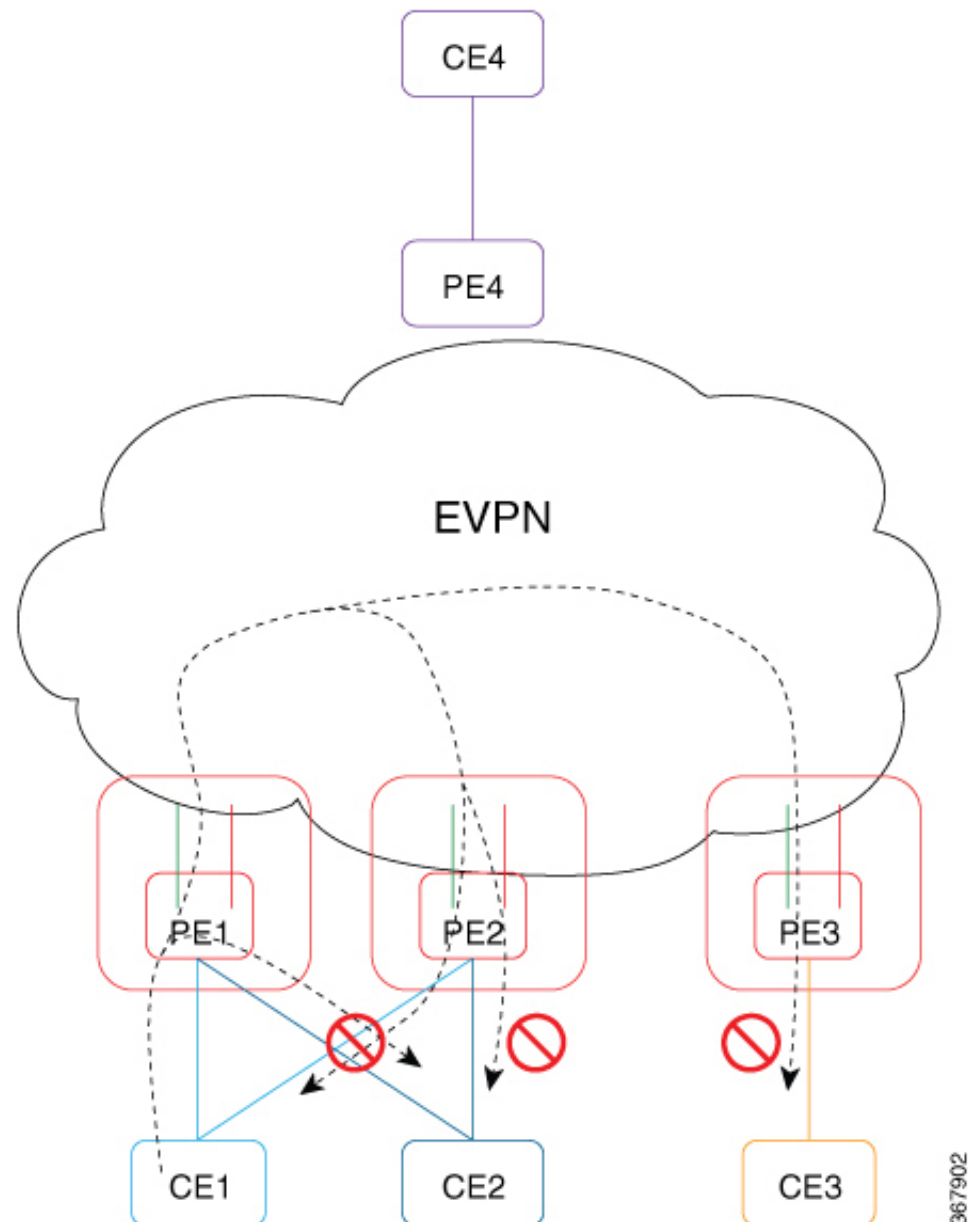
Figure 7: EVPN E-Tree
